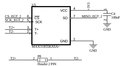
THERMOCOUPLE_2 SENSOR
