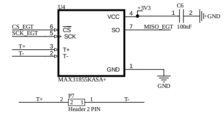
THERMOCOUPLE SENSOR
